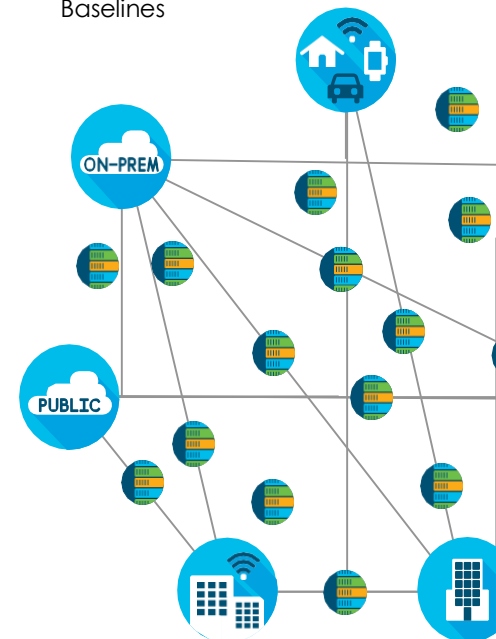
Key Vaults
